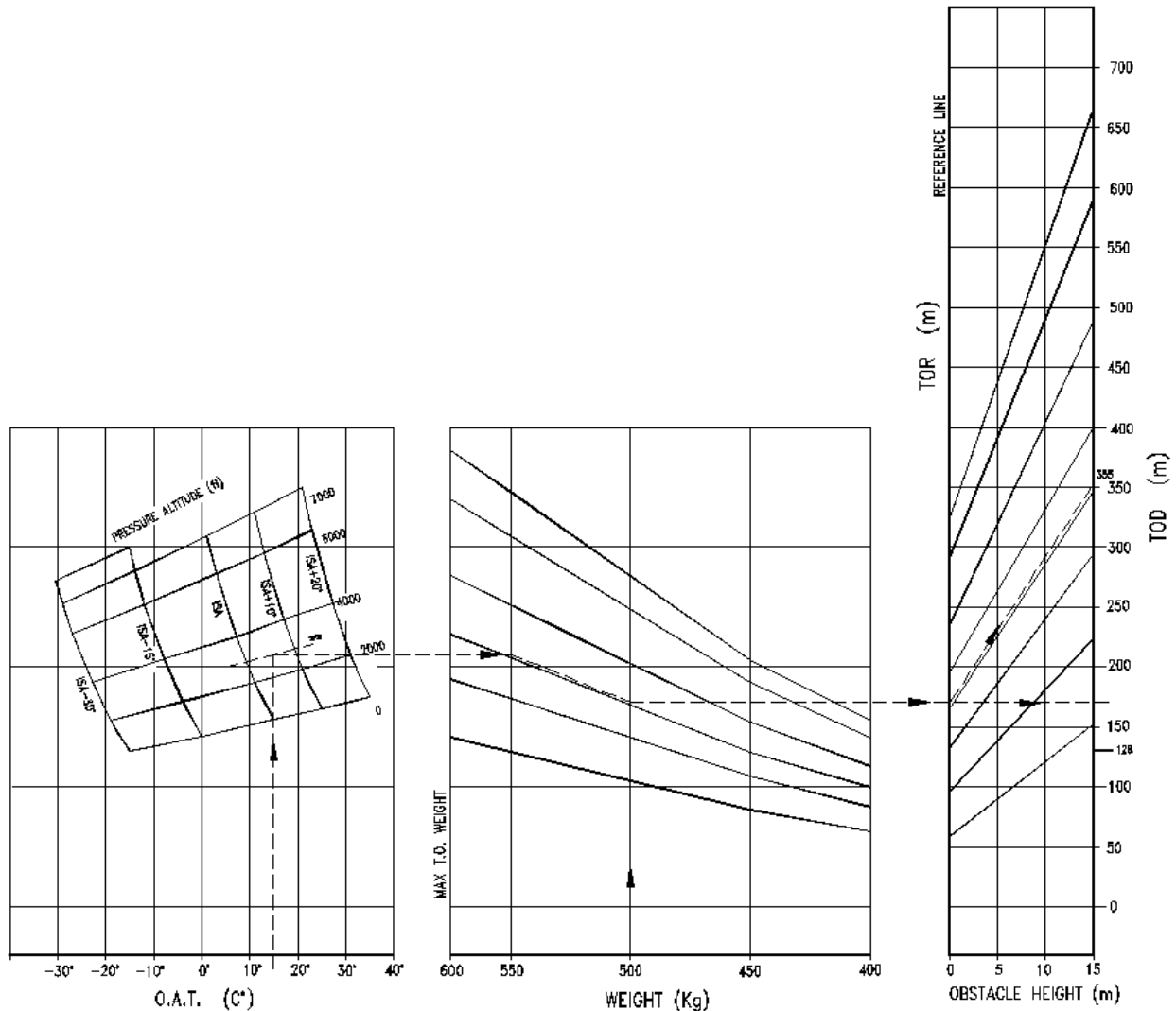
Fig. 4-4 Takeoff performance
