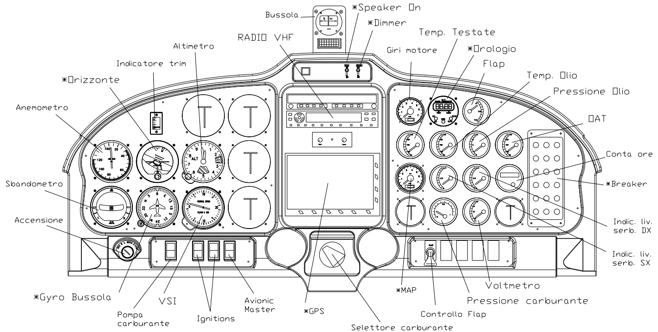
Fig. 1-2 Instrument Panel
