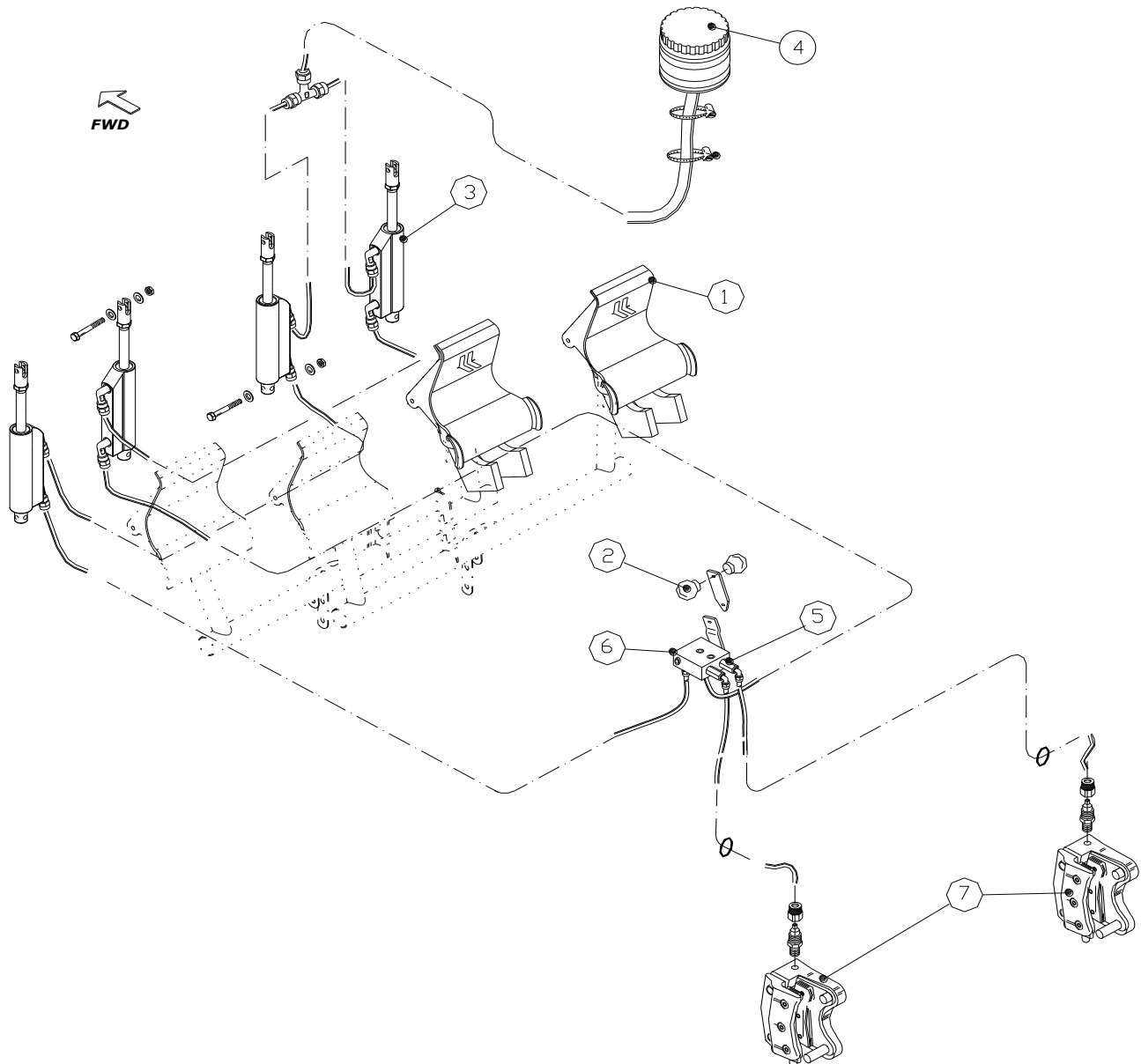
Fig. 1-7 Brake System
