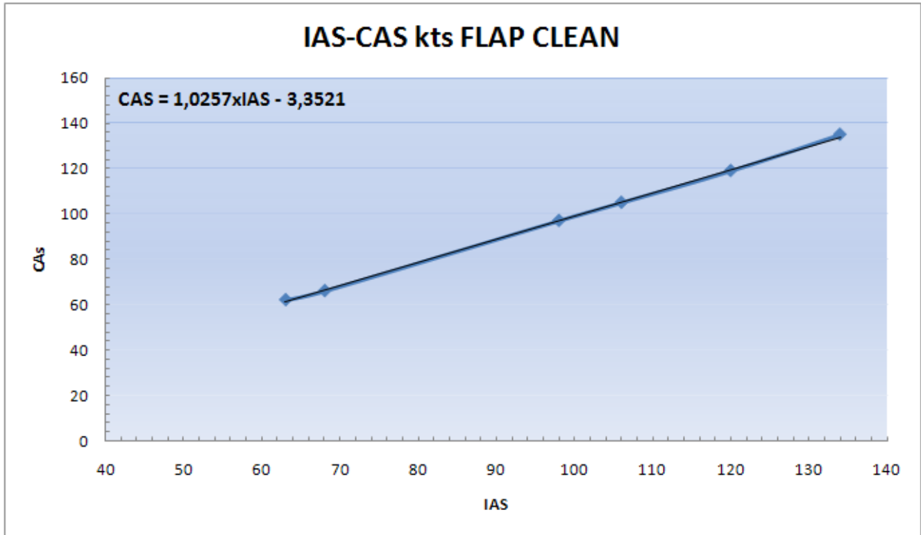
Fig. 4-1 Calibrated vs. Indicated Airspeed
