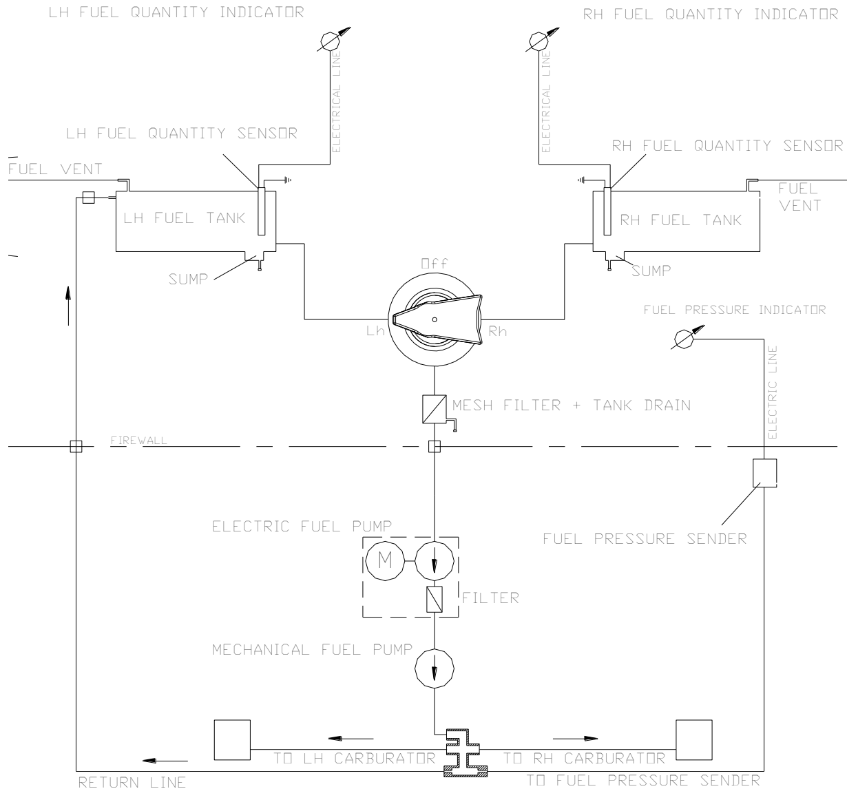
Figure 1-3 Fuel System
